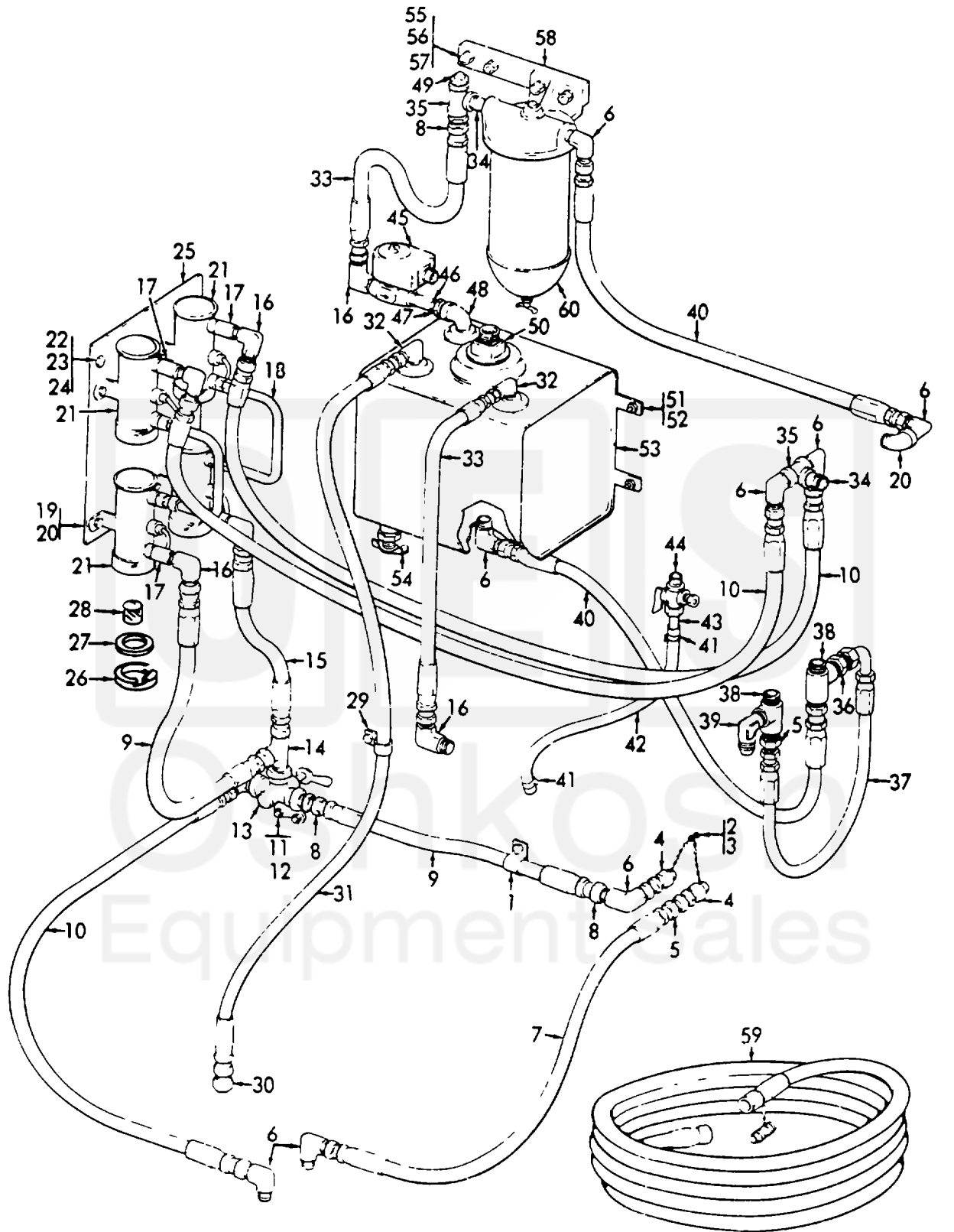
Figure 30. Fuel Lines, Valves, Pumps and Fittings.
